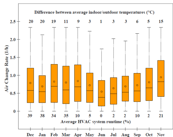
Figure 2. Monthly variation of ACR in the residence. December data (last 20 days of the month) shown are from 2016, while other months represent the data collected in 2017. On each boxplot, the central line indicates the median, the open circle indicates the mean, and the bottom and top edges of the box indicate the 25th and 75th percentiles, respectively.
