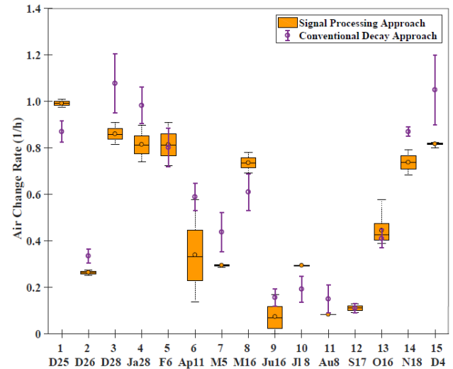
Figure 1. Comparison between the calculated air change rates from the signal processing approach and the conventional decay approach over 15 hourly decay periods from December 2016 to December 2017.
