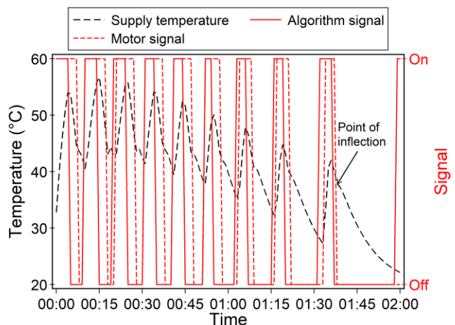
Figure 5 Temperature profile, On/Off signals recorded by motor sensor and calculated by the temperature method from Site 1, Toronto_B. Note fan continues to run after heating cycle ends.
