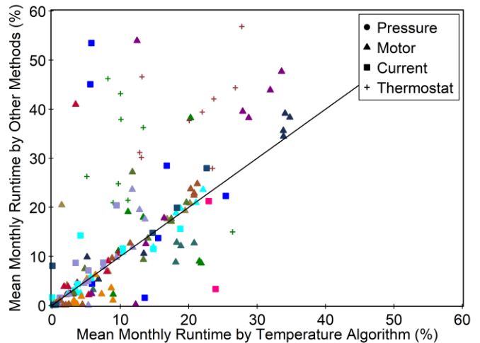
Figure 3 Comparison between mean monthly runtimes calculated by temperature algorithm and four other direct methods from 21 homes in Toronto, Ontario. The sites are differentiated by color.
